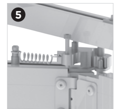
Ensemble de cames de compression
